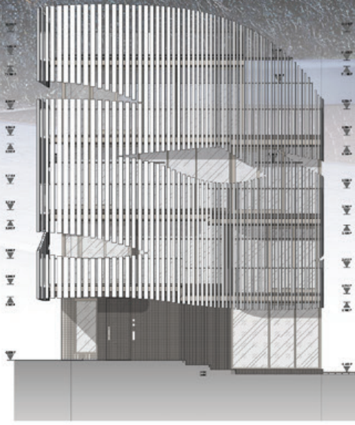
Elevation NE - side facade
