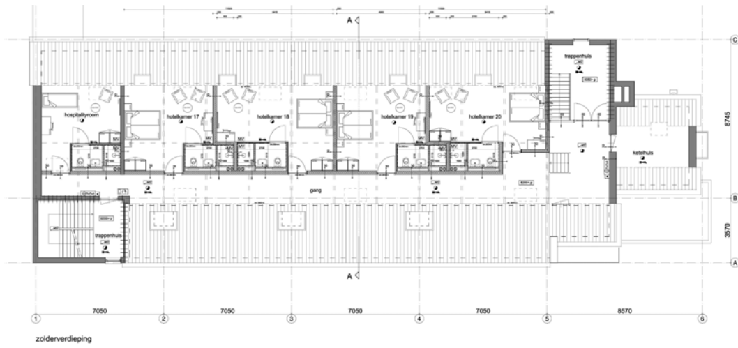
zolderverdieping
